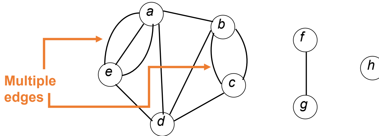
Graph G_2
