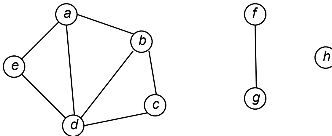
Graph G_1
