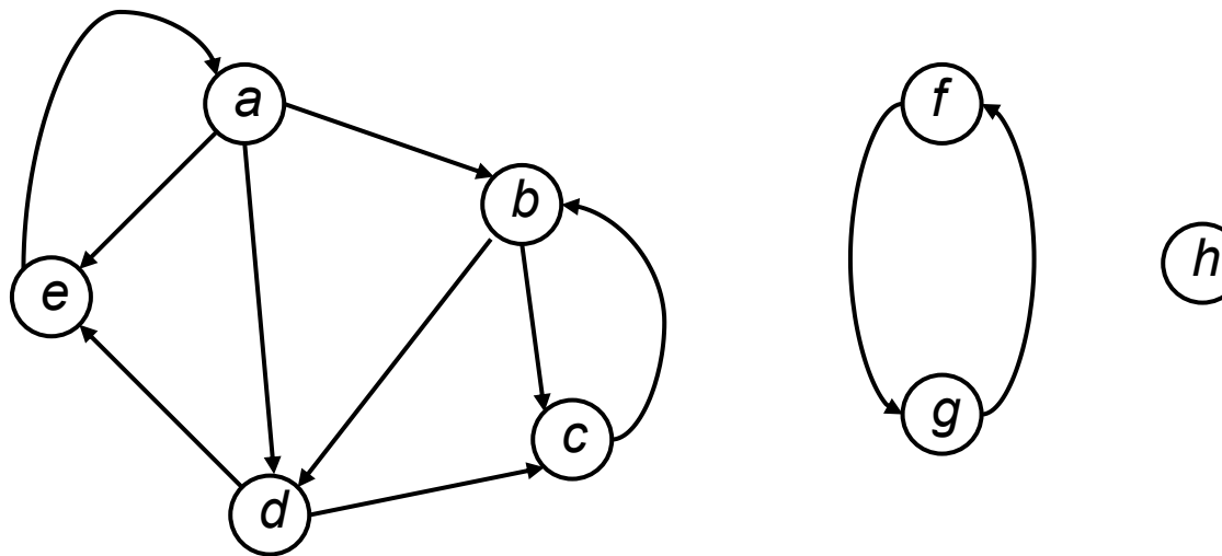
Graph G_3
