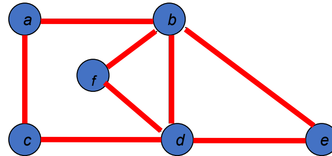
Euler graph
