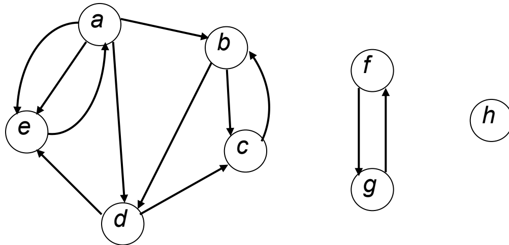
Graph G_4
